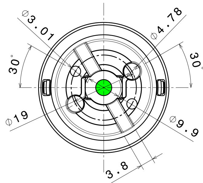
Rear view Scale: 3:2
